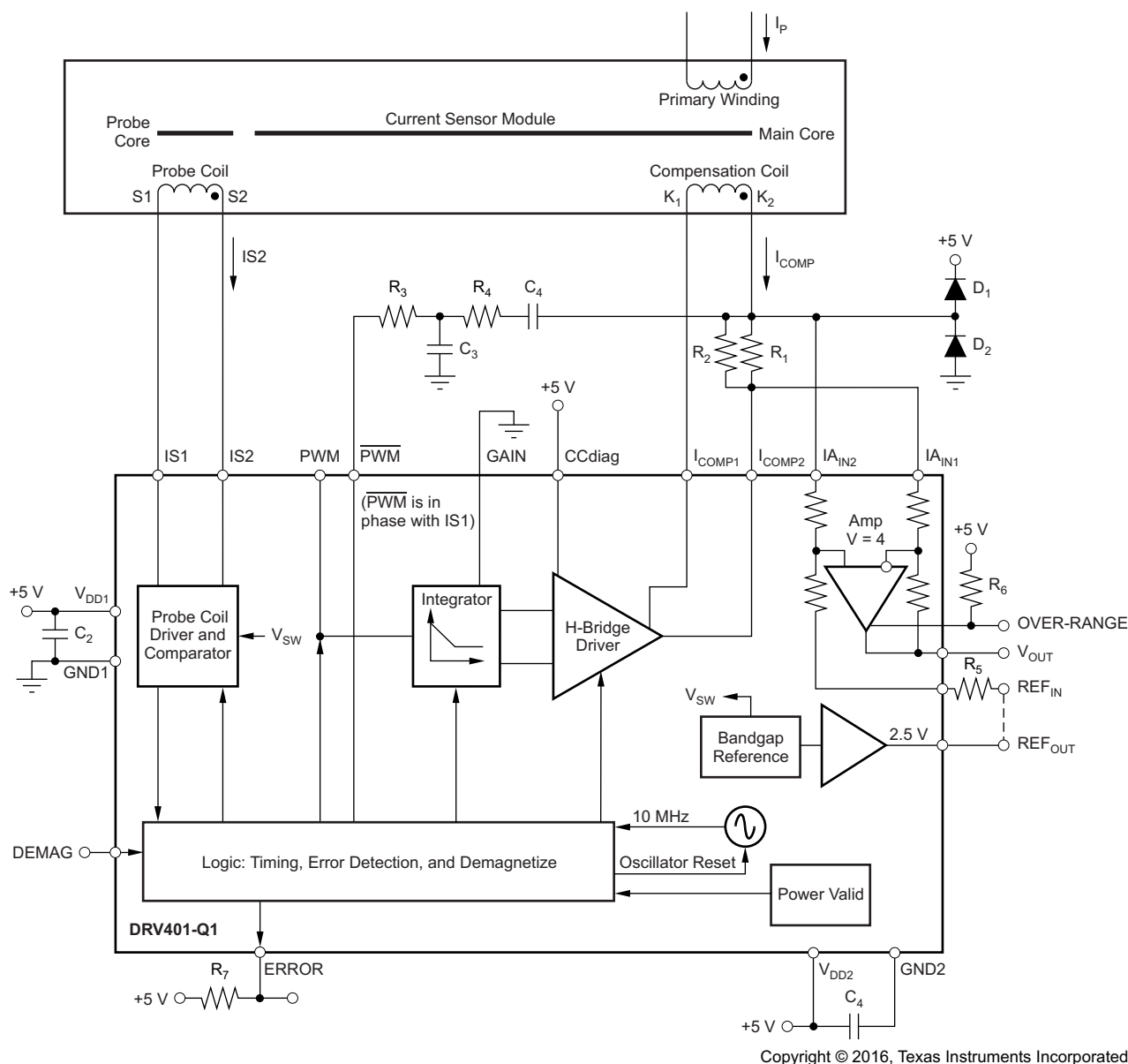
Figure 42. Basic Connection Circuit
