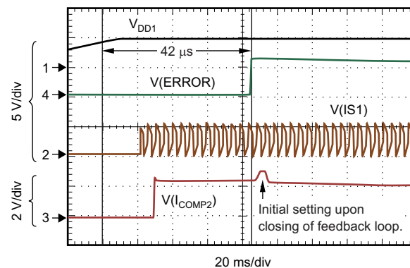
Figure 46. Demagnetization and Power-On Timing: Demagnetization Cycle on Power-Up
