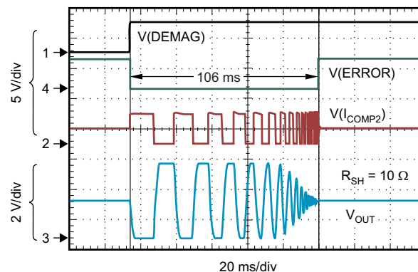
Figure 48. Demagnetization and Power-On Timing: Demagnetization Cycle On Command
