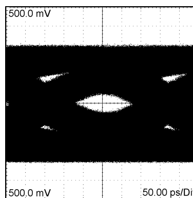
Figure 26. A 3.125 Gbps NRZ PRBS-23 without PE After 30\"
