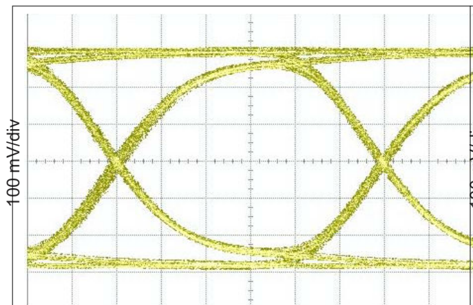
Figure 5-4. PRBS-7, Pre-Emphasis = 0 dB at 4 Gbps
