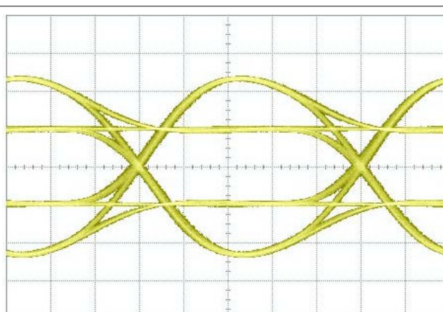
Figure 5-5. PRBS-7, Pre-Emphasis = -9 dB at 4 Gbps
