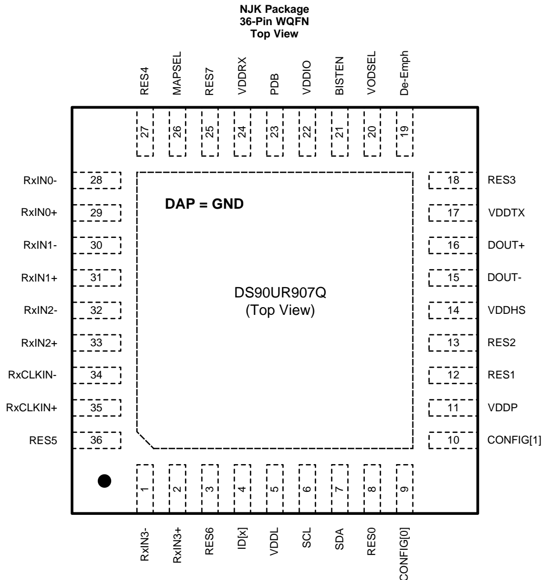
Pin Functions
