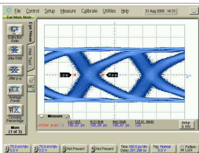
Serializer CML Output Stream with Input PÄCLK = 65 MHz, VODSEL = H
