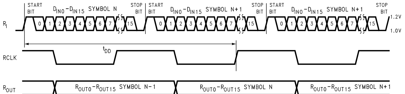
Figure 11. Deserializer Delay
