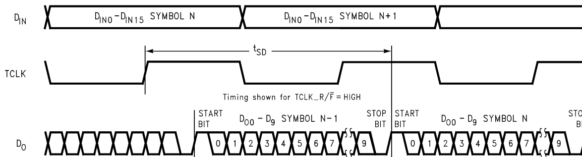
Figure 7. Serializer Delay
