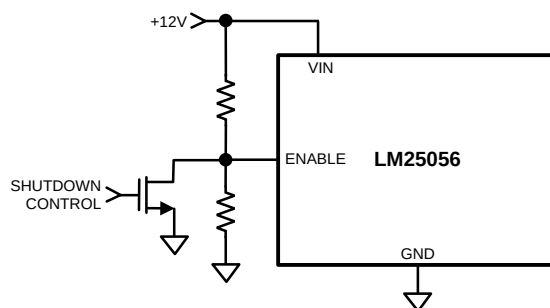
Figure 15. ENABLE Control
