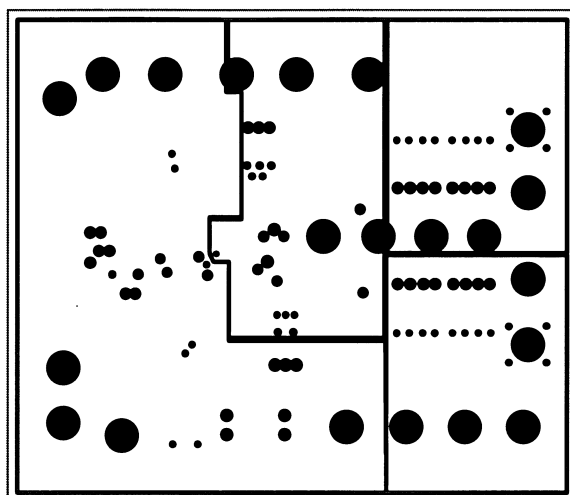
Figure 28. Internal Plane 2
