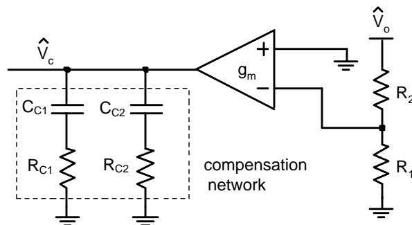
Figure 19. Compensation Network
