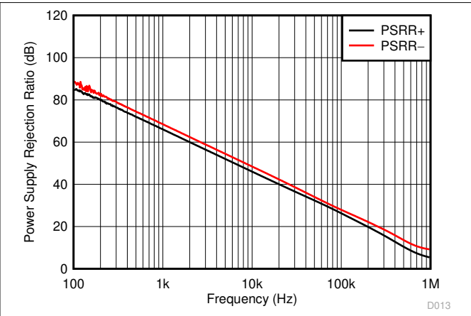
Figure 6-7. PSRR vs Frequency
