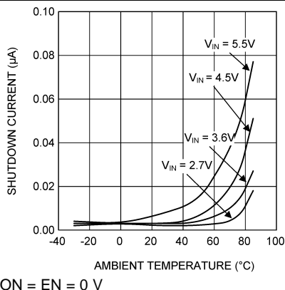
Figure 1. Shutdown Current vs Temperature
