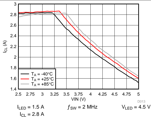
Figure 23. Inductor Current Limit vs Input Voltage
