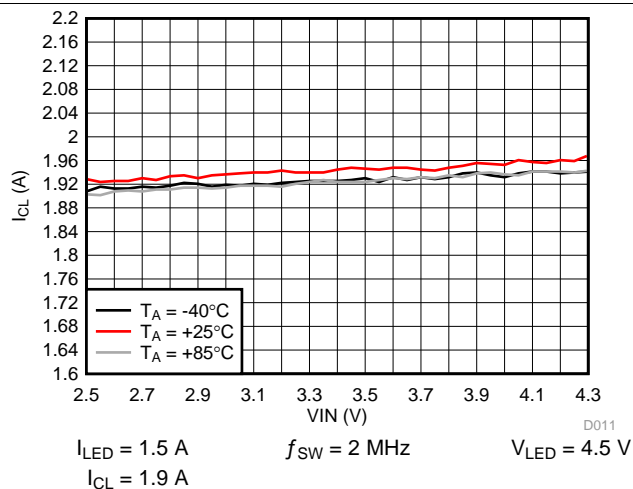
Figure 21. Inductor Current Limit vs Input Voltage
