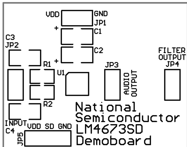
Composite View
