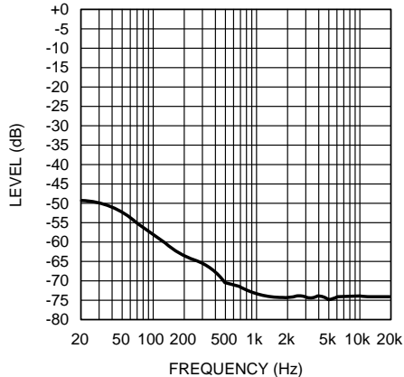
Figure 10. Input Floating
