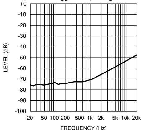
Figure 13. Input Floating
