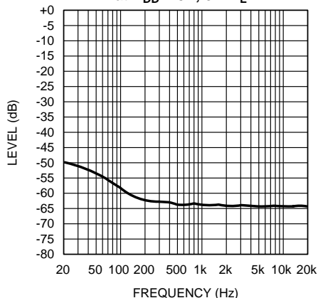
Figure 8. Input terminated with 10Ω
