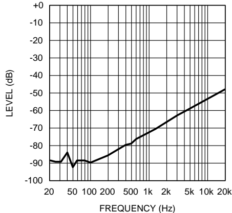
Figure 11. Input Floating
