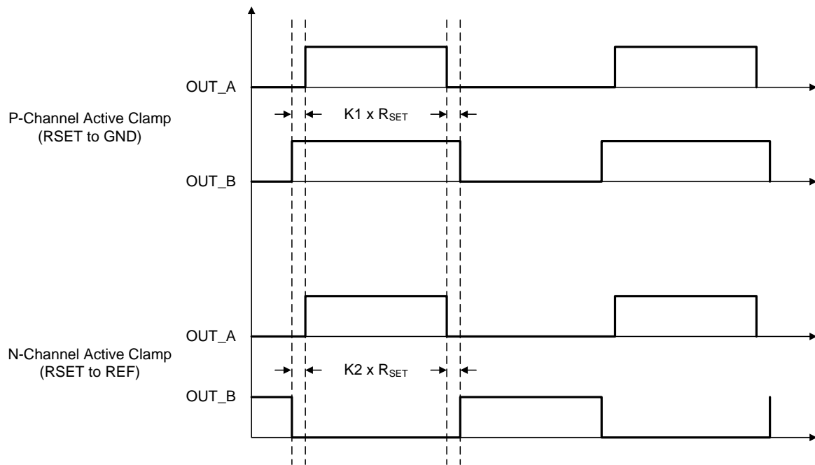
Figure 14. PWM Outputs
