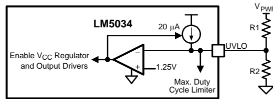
Figure 29. UVLO Circuit
