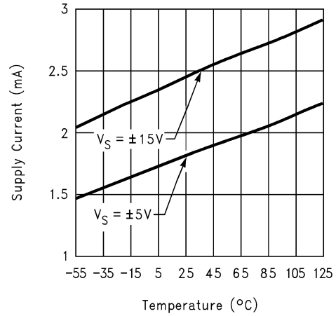
Figure 5-54. Supply Current vs Temperature
