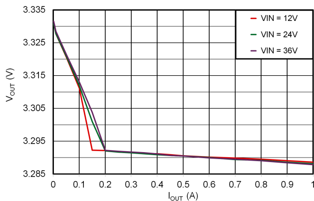
Figure 6-8. 3.3V Load Regulation
