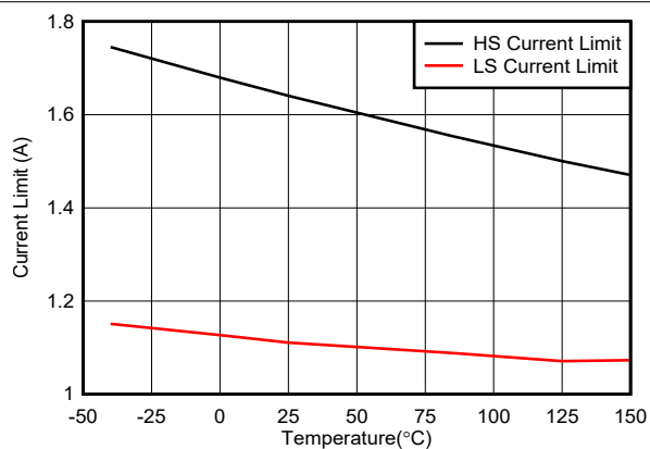
Figure 6-12. HS and LS Current Limit Versus Temperature
