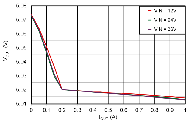
Figure 6-7. 5V load Regulation
