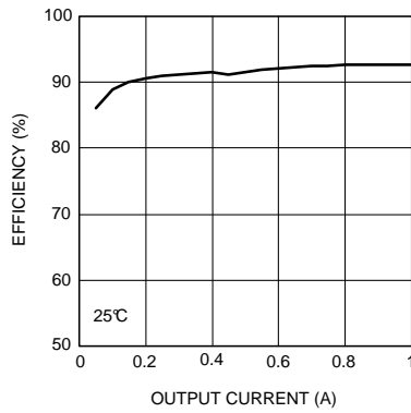
Figure 39. Efficiency
