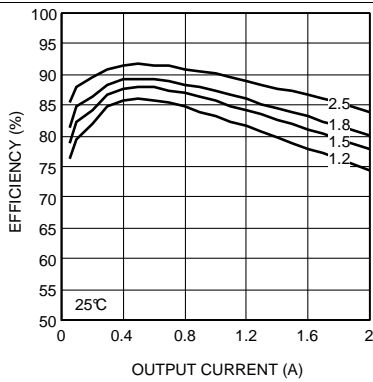
Figure 1. Efficiency 6-V Input
