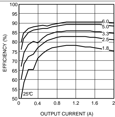
Figure 5. Efficiency 24-V Input
