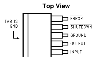
Figure 2. Plastic Surface Mount Package 5-Lead DDPak/TO-263 Package See Package Number KTT0005B
