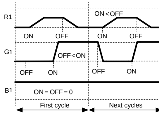
Figure 23. Example Blinking Waveforms
