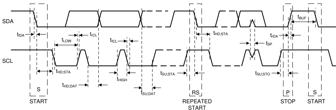
Figure 7-16. I²C-Compatible Timing
