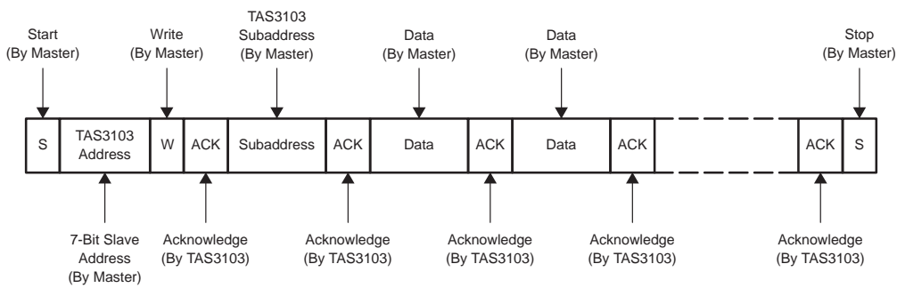
Figure 2–16. I 2 C Subaddress Access Protocol
