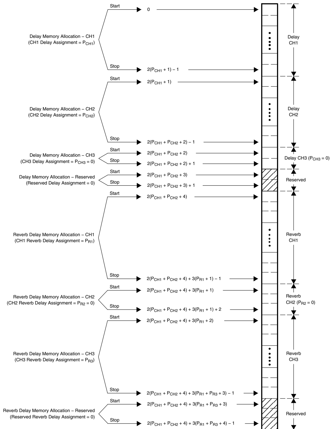
Figure 3–19. Delay-Line Memory Implementation
