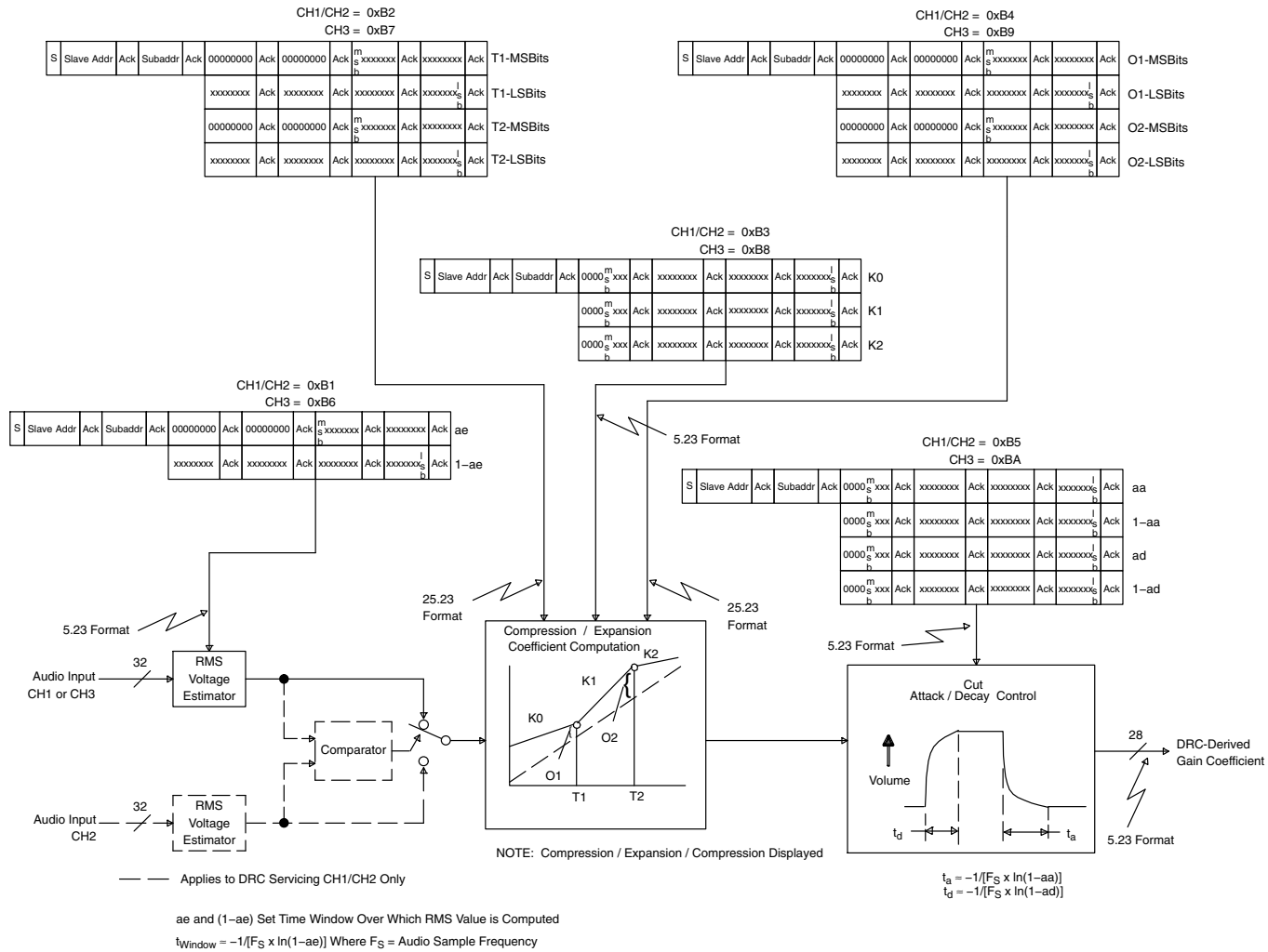
Figure 3-23. DRC Block Diagram
