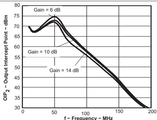
Figure 58. OIP 2 , dBm vs Frequency
