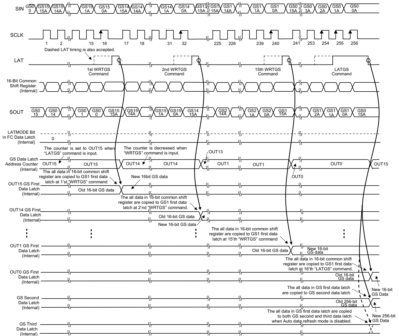
Figure 27. 256-Bit GS Data Write Sequence Timing Diagram (15 x WRTGS + 1 LATGS, LATMODE = 0)
