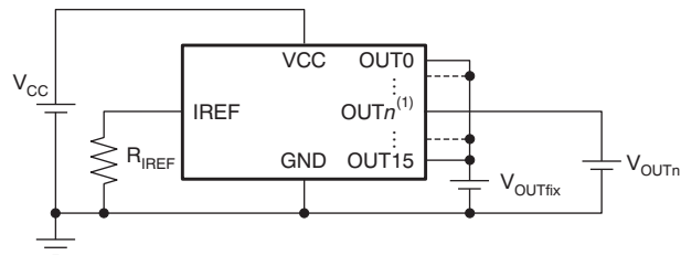
Figure 7. Constant-Current Test Circuit for OUT_n
