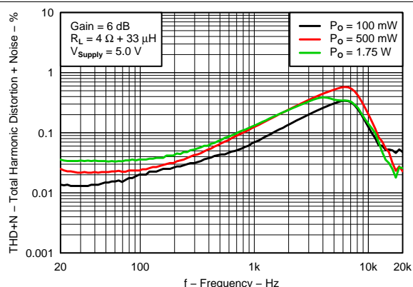
Figure 15. Total Harmonic Distortion + Noise vs Frequency V_{SUPPLY} = 5 \text{ V}, 4 \Omega
