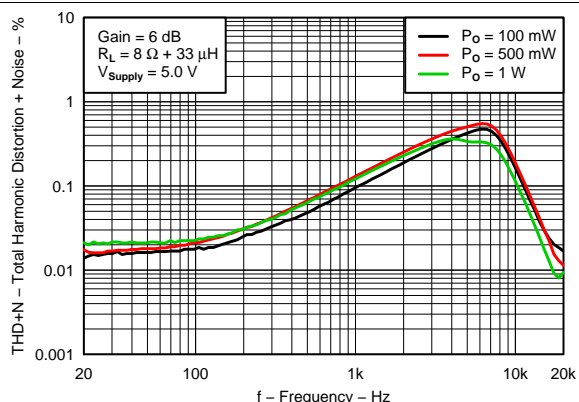
Figure 16. Total Harmonic Distortion + Noise vs Frequency V_{SUPPLY} = 5 \text{ V}, 8 \Omega
