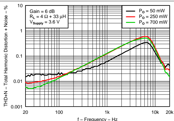
Figure 13. Total Harmonic Distortion + Noise vs Frequency V_{SUPPLY} = 3.6 \text{ V}, 4 \Omega
