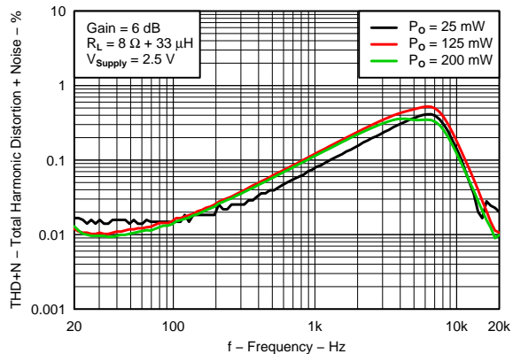
Figure 12. Total Harmonic Distortion + Noise vs Frequency V_{SUPPLY} = 2.5 \text{ V}, 8 \Omega
