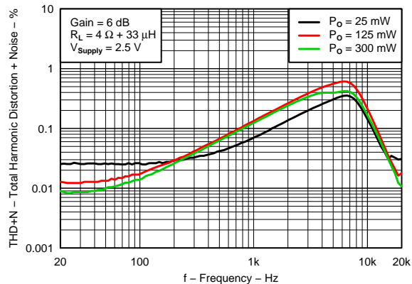
Figure 11. Total Harmonic Distortion + Noise vs Frequency V_{SUPPLY} = 2.5 \text{ V}, 4 \Omega
