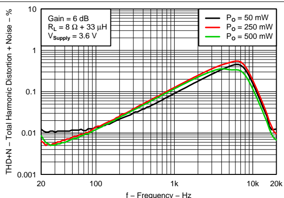
Figure 14. Total Harmonic Distortion + Noise vs Frequency V_{SUPPLY} = 3.6 \text{ V}, 8 \Omega
