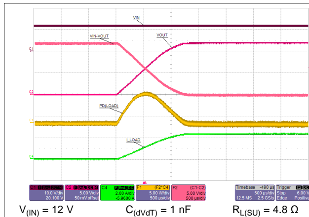
Figure 55. Start-up With Load
