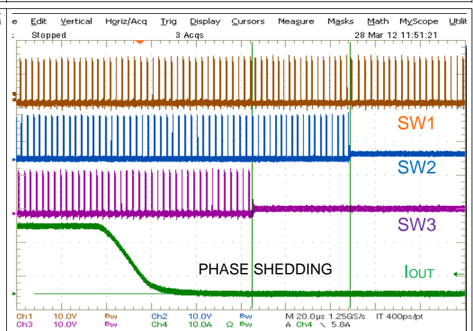
Figure 116. Phase Shedding
