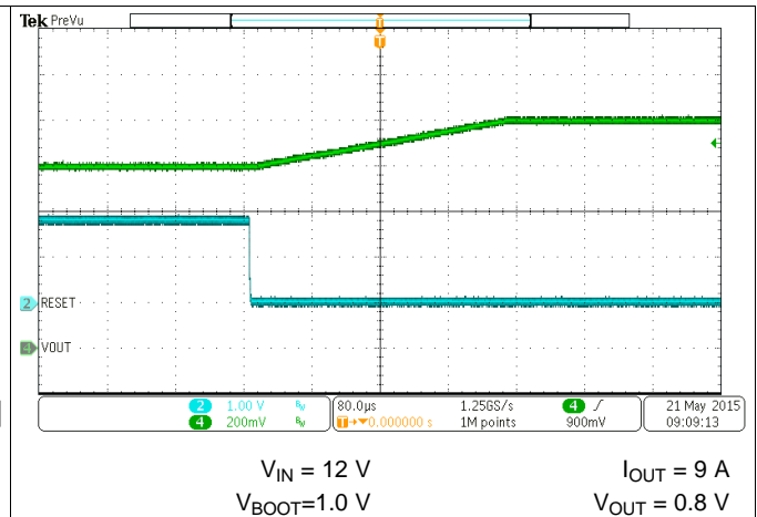
Figure 112. RESET Function ( V_{OUT}=0.8\text{ V} )
