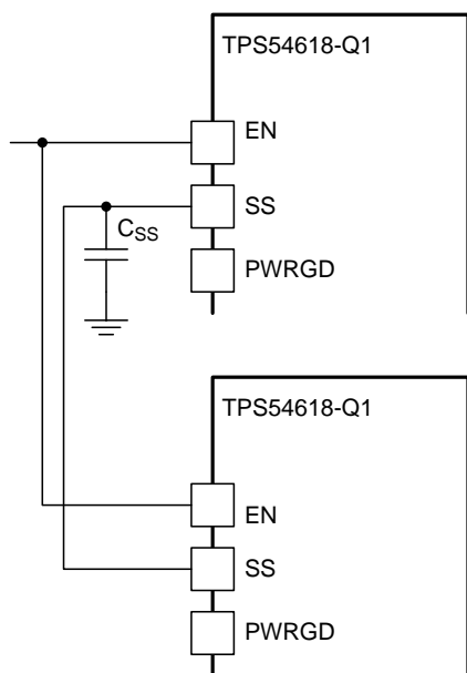
Figure 29. Schematic for Ratio-Metric Start-Up Sequence
