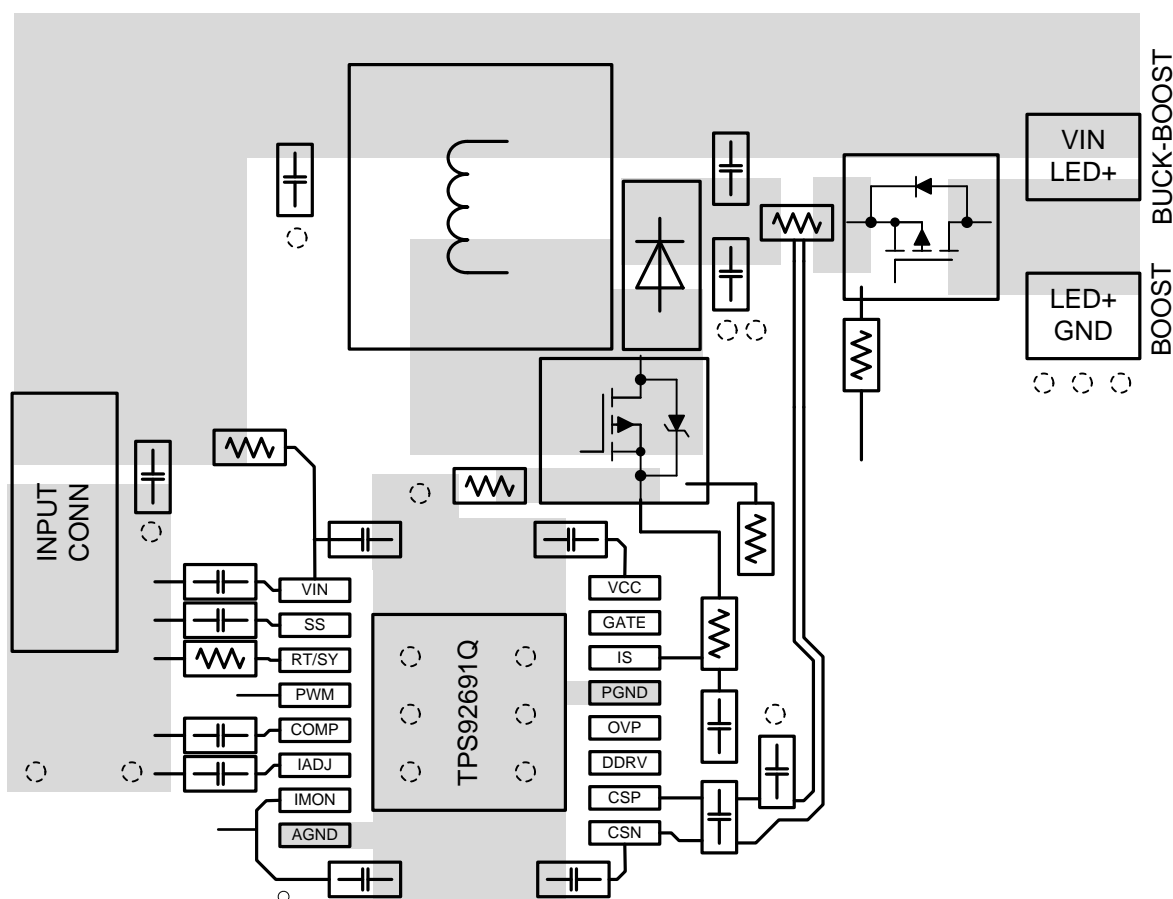
Figure 45. Layout Recommendation
