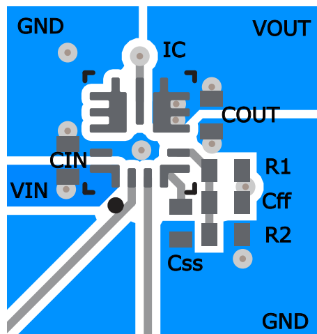
Figure 9-33. Example Layout
