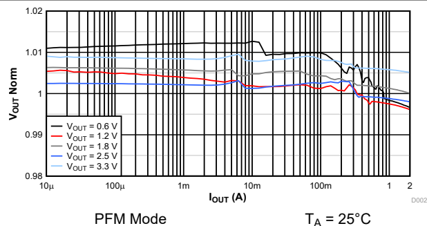
Figure 9-14. Load Regulation V_{IN} = 5\text{ V}
