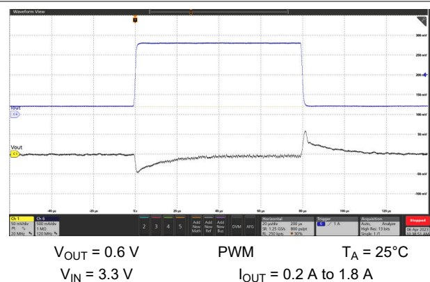
Figure 9-16. Load Transient Response
