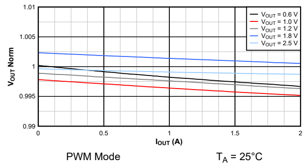
Figure 9-13. Load Regulation V_{IN} = 3.3\text{ V}
