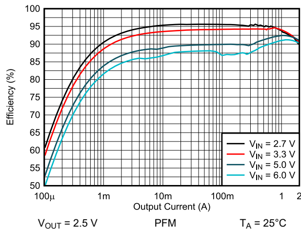
Figure 9-4. Efficiency versus Output Current
