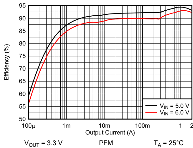
Figure 9-2. Efficiency versus Output Current
