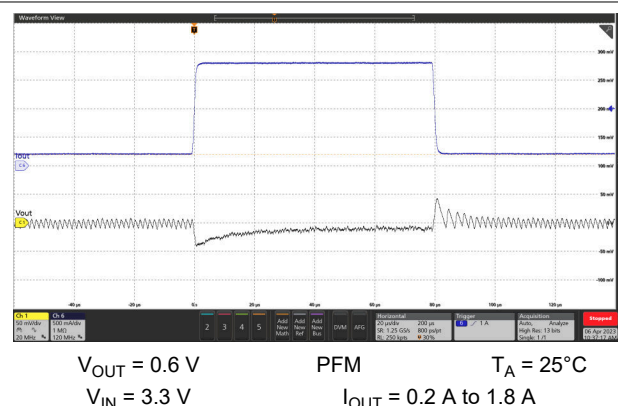
Figure 9-17. Load Transient Response
