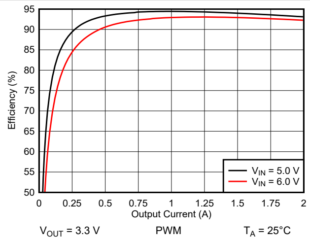
Figure 9-3. Efficiency versus Output Current
