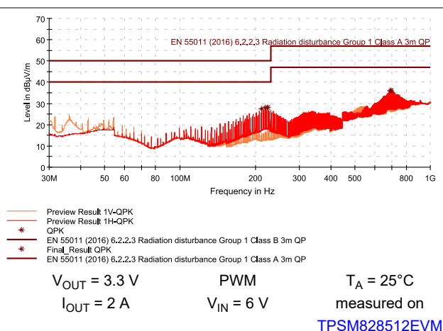
Figure 9-27. Radiated Emissions
