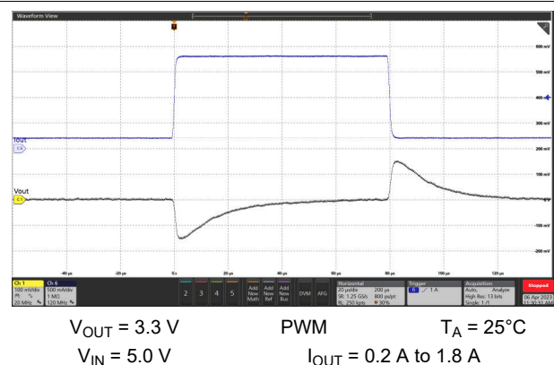
Figure 9-18. Load Transient Response
