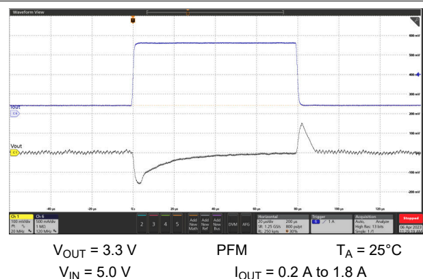
Figure 9-19. Load Transient Response
