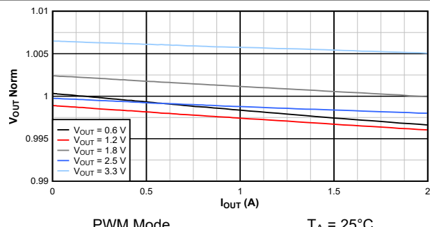
Figure 9-15. Load Regulation V_{IN} = 5\text{ V}
