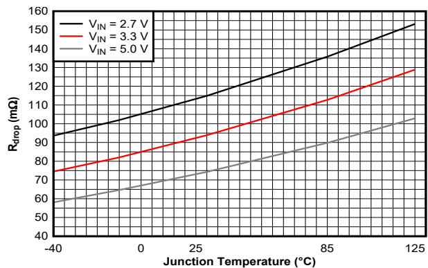
Figure 6-1. Dropout Resistance
