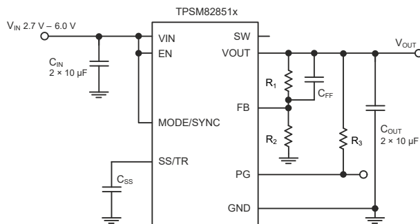
Simplified Schematic
