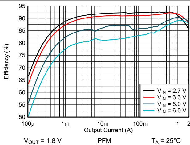
Figure 9-6. Efficiency versus Output Current
