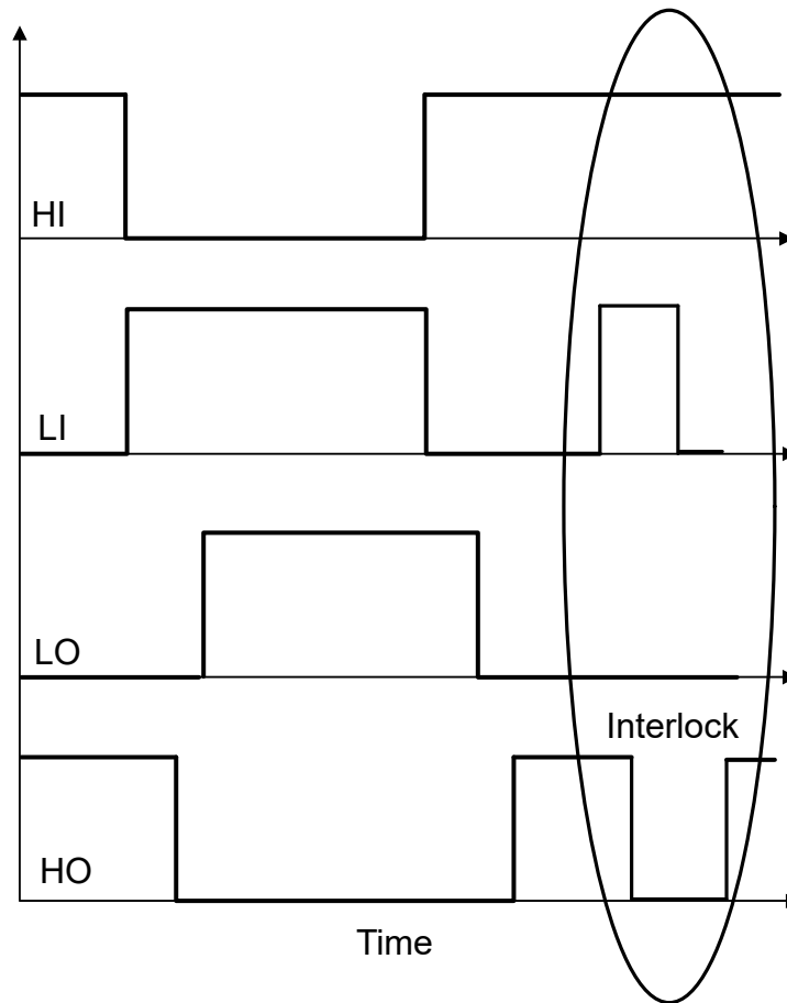
Figure 8-1. Interlock or Input Shoot-Through Protection
