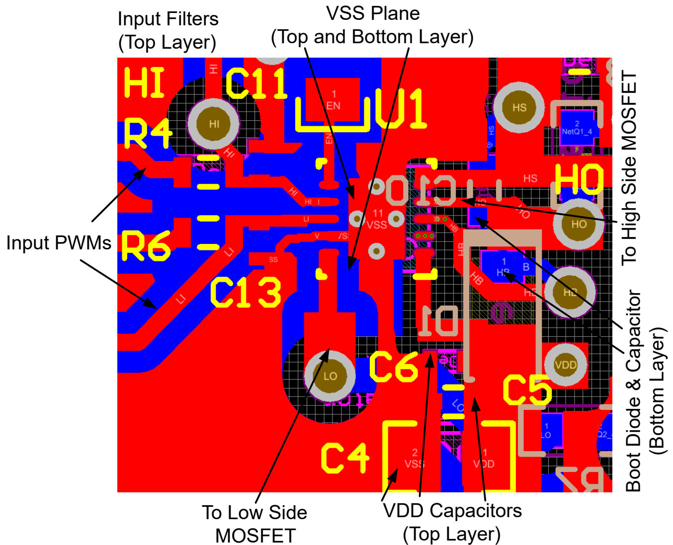
Figure 11-2. UCC27301A-Q1 PCB Layout Example for VSON package
