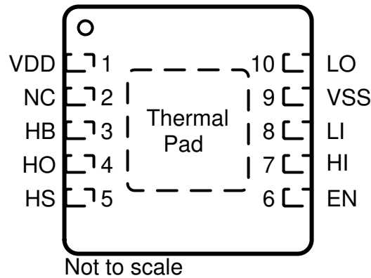
Figure 6-2. DRC Package 10-Pin SON Top View
