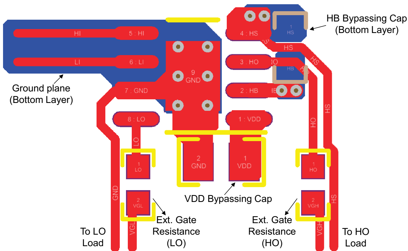
Figure 11-1. UCC27301A-Q1 PCB Layout Example for SOIC package
