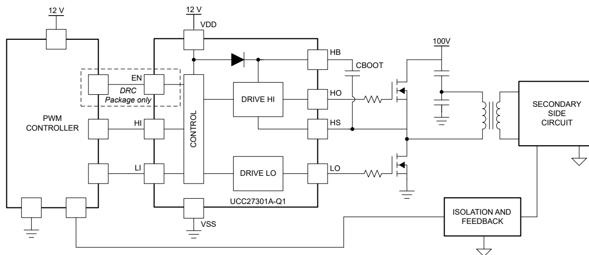
Figure 9-1. UCC27301A-Q1 Typical Application Diagram
