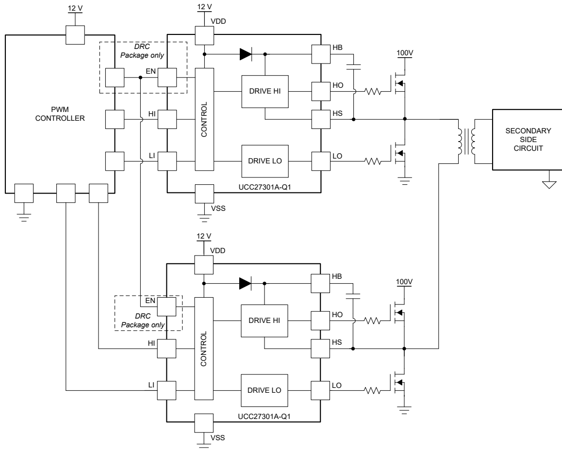
Figure 9-2. UCC27301A-Q1 Automotive Typical Application Diagram
