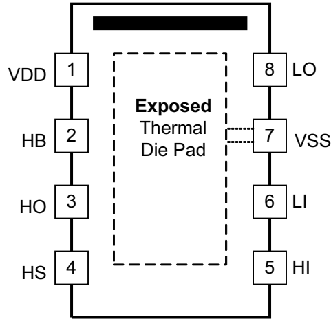
Figure 6-1. DDA Package 8-Pin SOIC with PowerPad™ Top View
