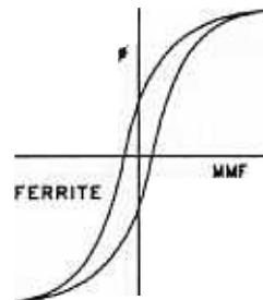
Fig 2. - Core Flux vs. Magnetic Force
