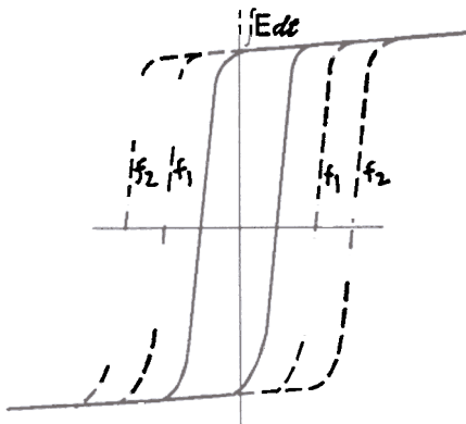
Fig 10. - L.F. Hysteresis plus Eddy Current
