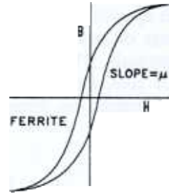
Fig 1. - Magnetic Core B-H Characteristic
