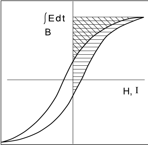
Fig. 1. B-H characteristics.
