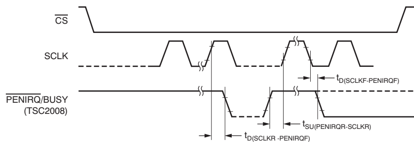
Figure 2. PENIRQ Timing
