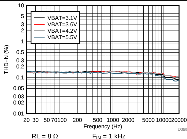
Figure 37. si-sense THD+N vs Frequency
