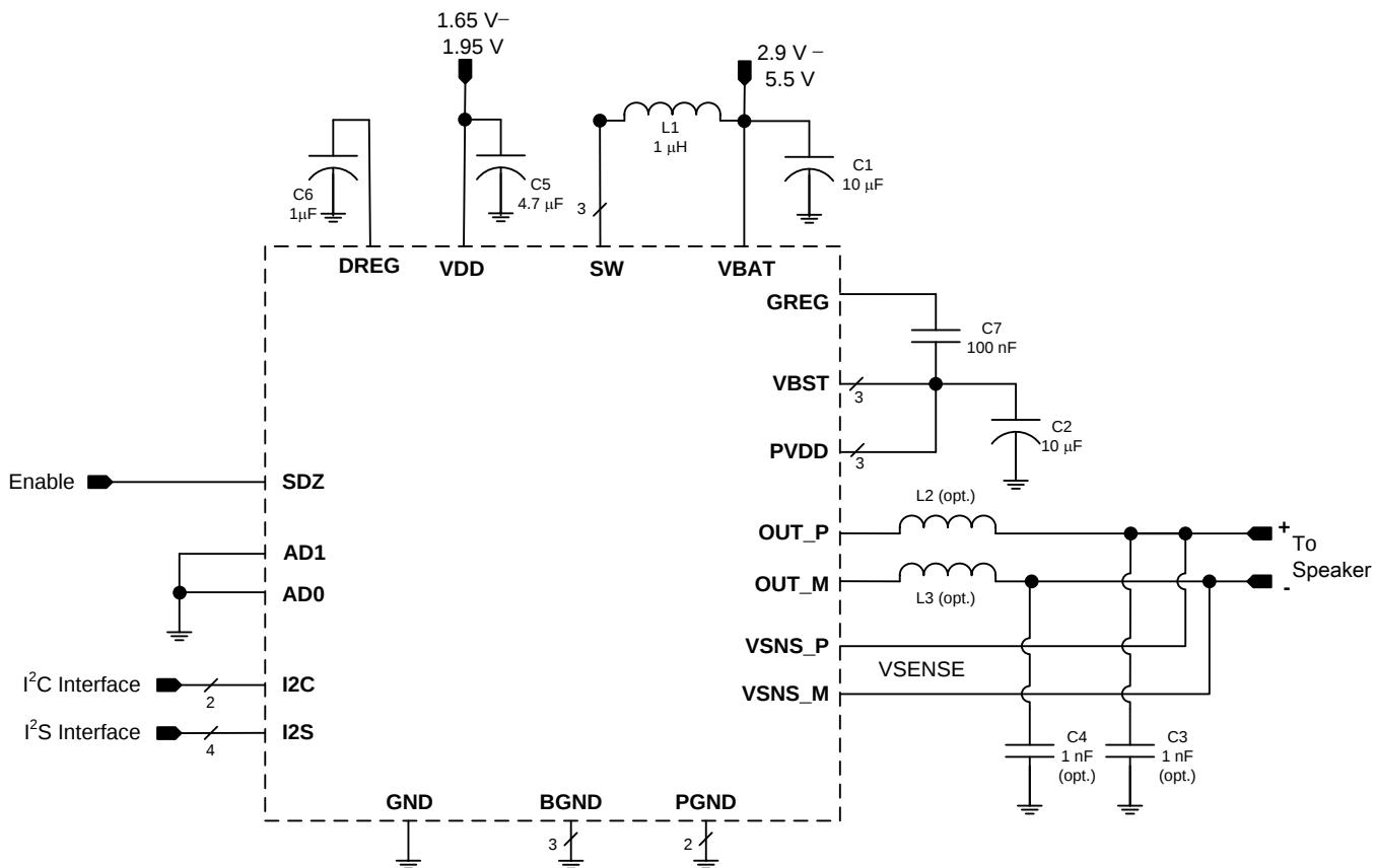
Figure 69. Typical Application - Digital Audio Input
