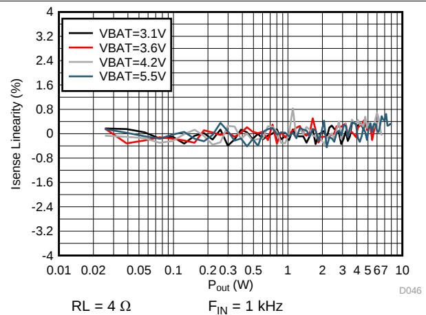
Figure 40. V-sense Linearity vs Output Power
