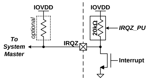
Figure 55. IRQZ Pin
