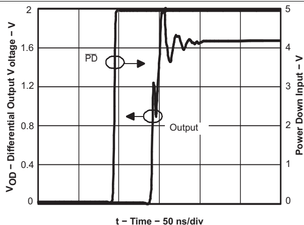
Figure 31. Turnon Time
