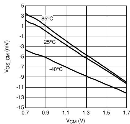
Figure 5-44. V_{OS\_CM} vs V_{CM}
