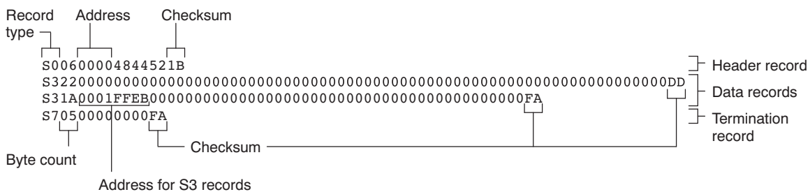
Figure 12-11. Motorola-S Format
