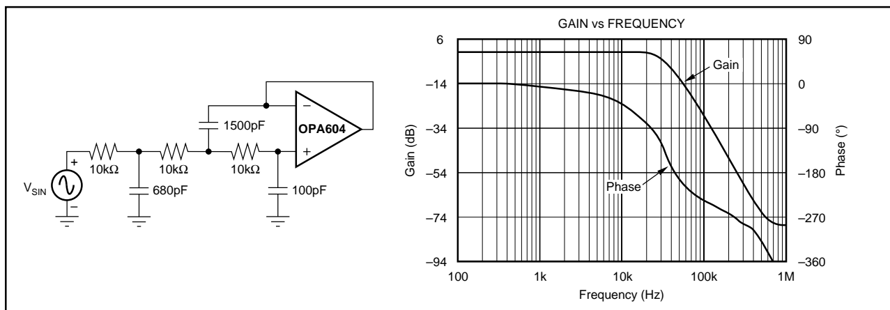
FIGURE 14. 3rd-Order LPF.
