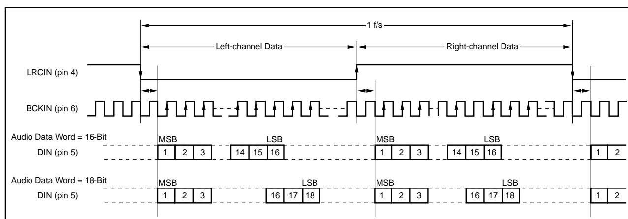
FIGURE 4. "I²S" Data Input Timing.
