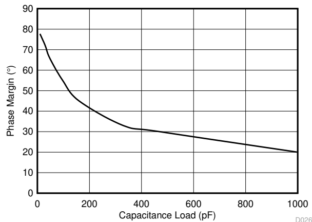
Figure 6-21. Phase Margin vs Capacitive Load
