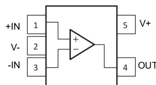
Figure 5-2. LMV321A DCK Package, 5-Pin SOT-23, SC70 (Top View)
