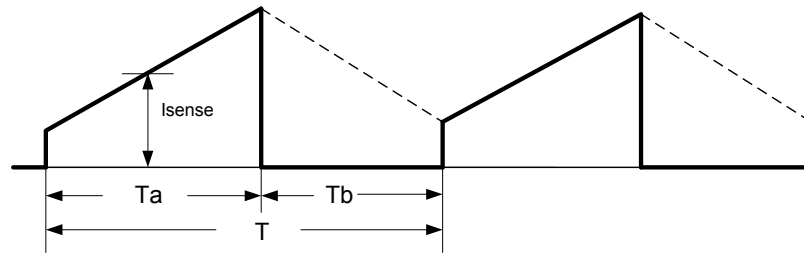
Figure 4a. Sensed current waveform at continuous conduction mode
