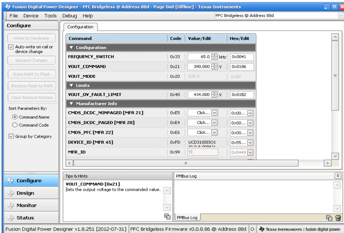
Figure 9. Configure PFC Operation Setpoints
