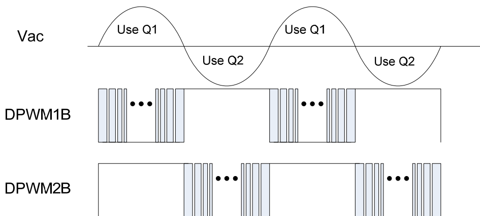
Figure 3. PWM waveform for bridgeless PFC
