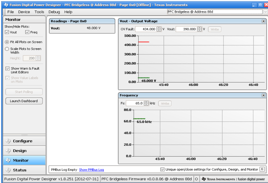
Figure 8. Monitor PFC Operating Status
