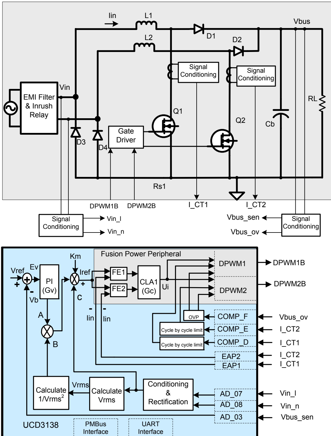
Figure 1. UCD3138 controlled bridgeless PFC block diagram
