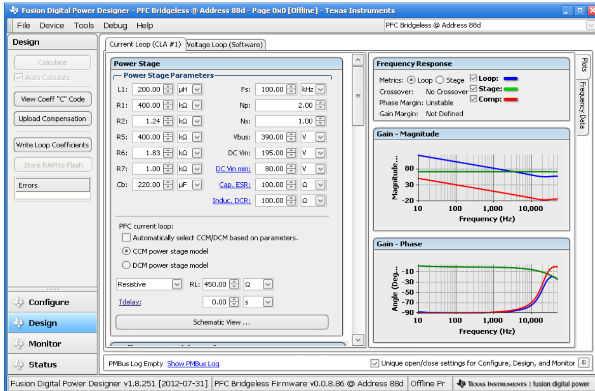
Figure 10. Tune PFC Control Loop
