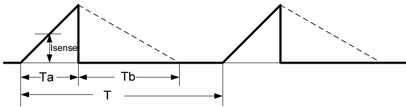
Figure 4b. Sensed current waveform at discontinuous conduction mode
