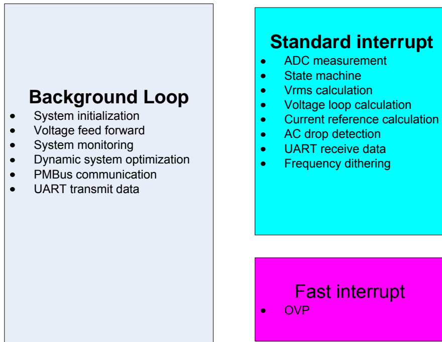
Figure 6. Firmware Structure
