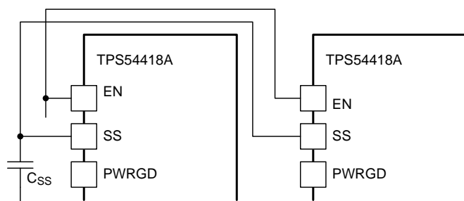
Figure 25. Sequential Start-Up Schematic
