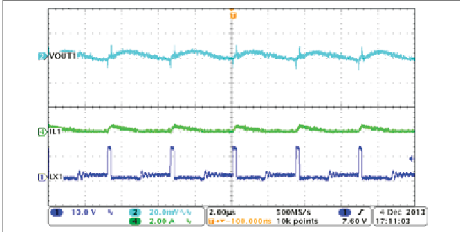
Figure 8-9. Buck1, Steady State Operation With Light Load
