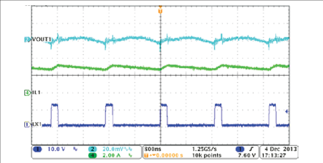
Figure 8-10. Buck1, Steady State Operation With Full Load
