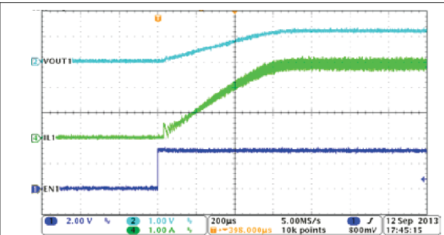
Figure 8-4. Buck1, Soft-Start With Full Load
