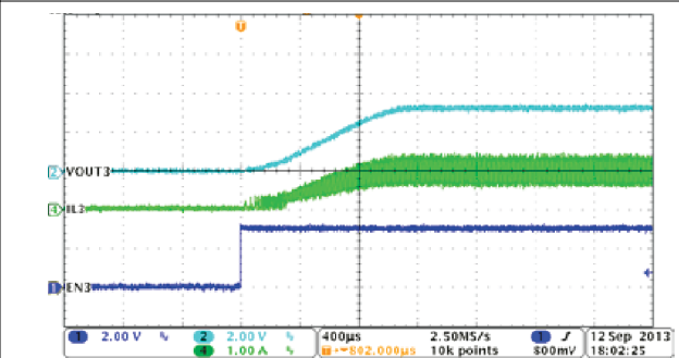
Figure 8-8. Buck3, Soft-Start With Full Load
