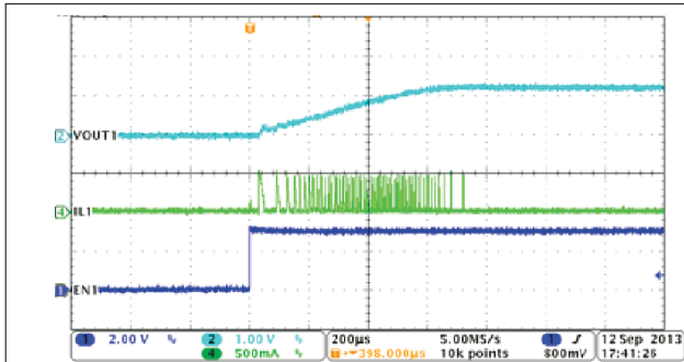
Figure 8-3. Buck1, Soft-Start With No Load
