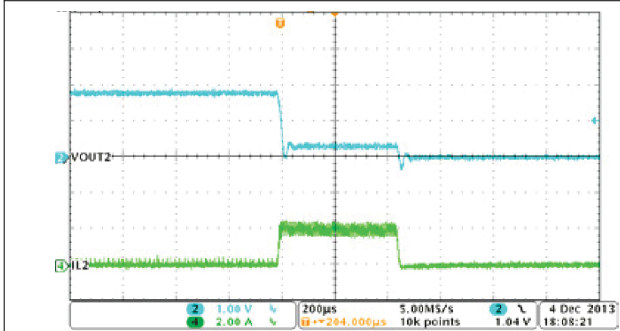
Figure 8-23. Buck2, Overcurrent Protection
