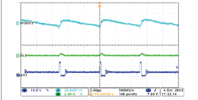
Figure 8-13. Buck3, Steady State Operation With Light Load
