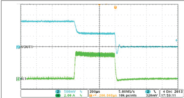
Figure 8-21. Buck1, Overcurrent Protection
