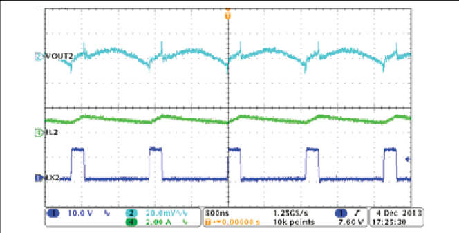
Figure 8-12. Buck2, Steady State Operation With Full Load
