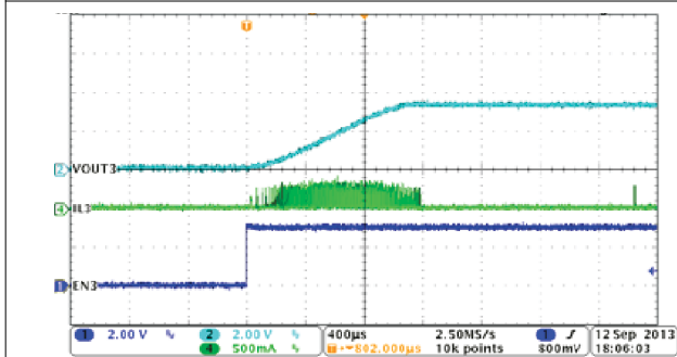
Figure 8-7. Buck3, Soft-Start With No Load
