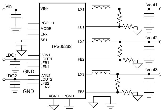
Application Schematic
