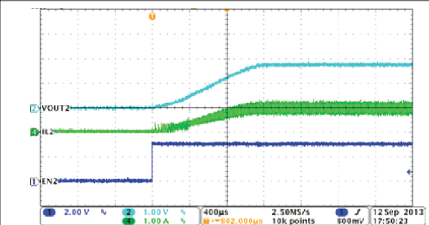
Figure 8-6. Buck2, Soft-Start With Full Load
