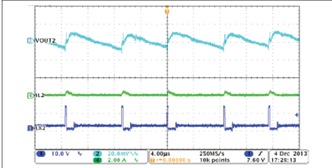
Figure 8-11. Buck2, Steady State Operation With Light Load
