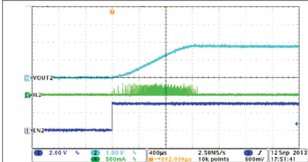
Figure 8-5. Buck2, Soft-Start With No Load
