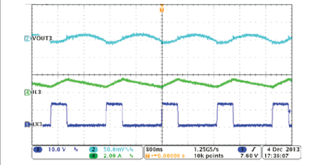
Figure 8-14. Buck3, Steady State Operation With Full Load
