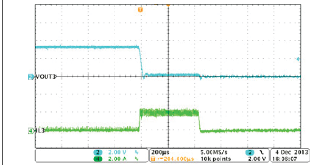
Figure 8-25. Buck3, Overcurrent Protection
