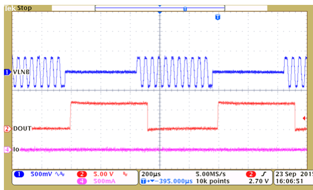
Figure 8-19. DOUT Tone Detection Output
