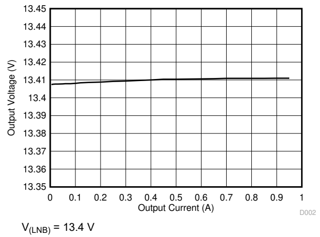
Figure 6-2. Load Regulation
