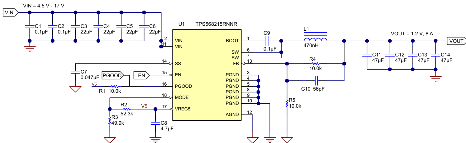
Figure 8-1. Application Schematic
