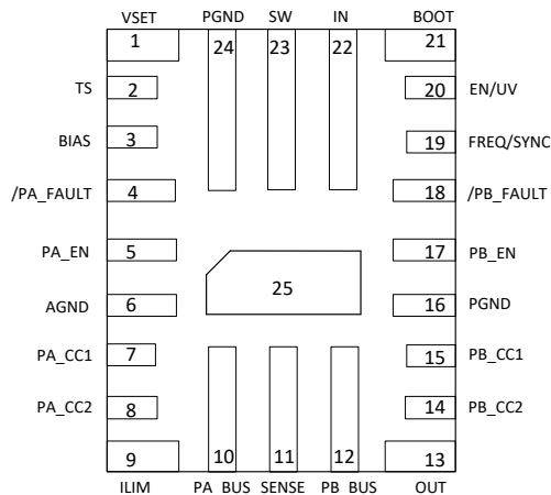
Figure 7-3. TPS25852-Q1 RPQ Package 25-Pin (QFN) Top View
