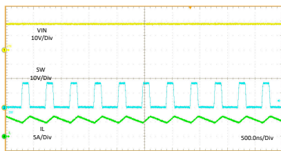
Figure 10-5. Switching Frequency When R_{FREQ} = 8.45 \text{ k}\Omega
