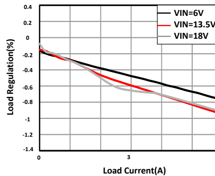
Figure 11-5. Load Regulation
