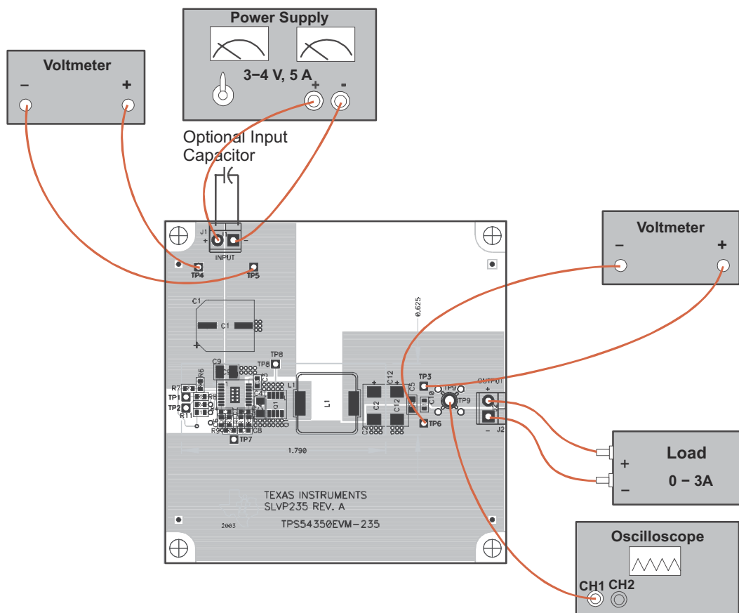
Figure 2-1. Connection Diagram
